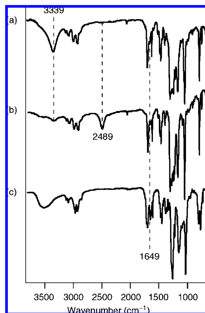
Figure 3. (a) IR spectrum of 2\cdot\text{CF}_3\text{SO}_3 as a KBr disk. (b) IR spectrum of D-labeled 2\cdot\text{CF}_3\text{SO}_3 as a KBr disk. (c) IR spectrum of 3\cdot\text{CF}_3\text{SO}_3 as a KBr disk. A broad peak at around 3500\text{ cm}^{-1} was derived from water.
