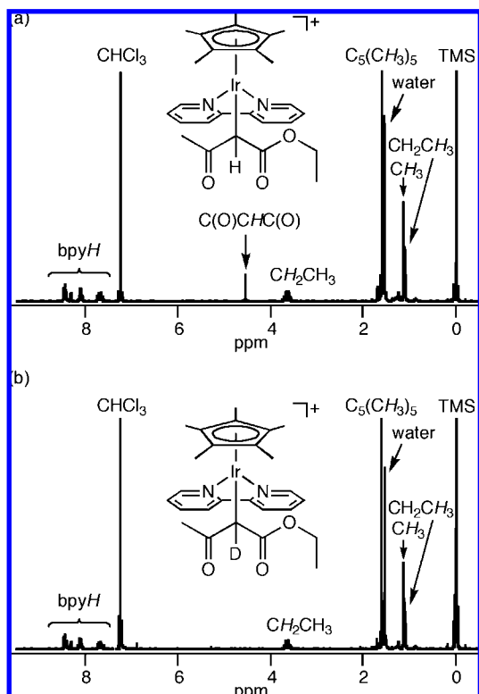
Figure 4. ^1\text{H} NMR spectra of 3\cdot\text{PF}_6 (a) and D-labeled 3\cdot\text{PF}_6 (b) in \text{CDCl}_3 at 25\text{ }^\circ\text{C} . TMS, reference with the methyl proton resonance set at 0.00\text{ ppm} .
