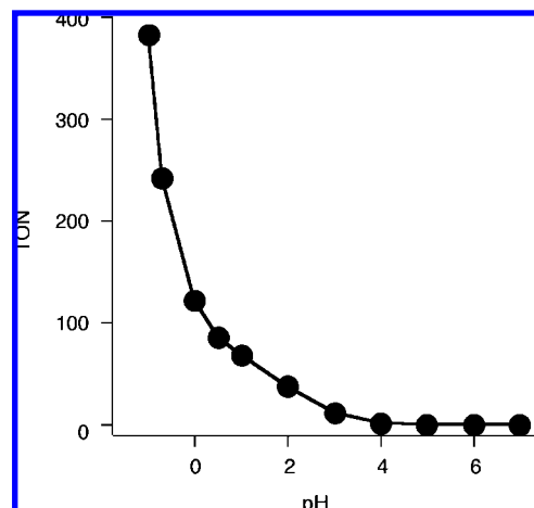
Figure 9. The pH-dependent TONs of the formation of ethyl acetoacetate in the reaction of 1 · \text{SO}_4 (0.2 μmol) with tetrolic acid ethyl ester (0.1 mmol) in \text{H}_2\text{O} (2.0 mL) at 25 °C for 1 h.
